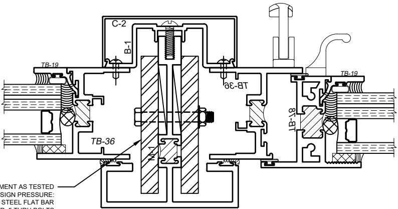
SECTION A: STEEL REINFORCEMENT
