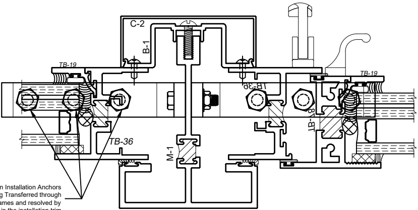
SECTION B: ANCH4 (HEAD SIMILAR)
